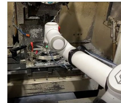
Loading and unloading of gears with machine tending
