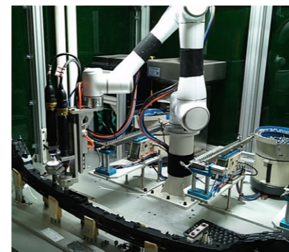
Taillights screwing
